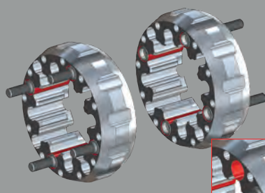
PERFIL I SPECIAL HOLES FOR M12 BOLTS
