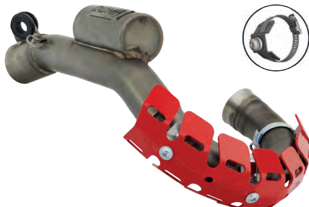
4 STROKE EVO SKU: 2CP0730003_ with clamp "easy fixing"
